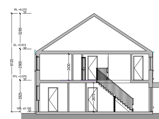
7 Section 1:200
