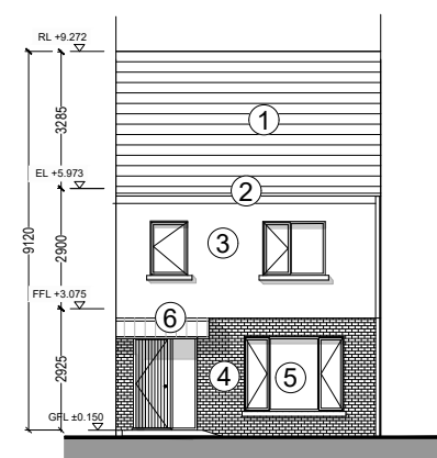
4 Front Elevation 1:200
