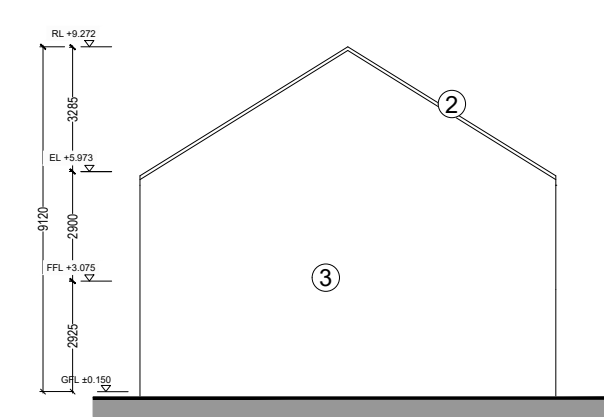
6 Side elevation 1:200
