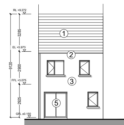
5 Rear Elevation 1:200
